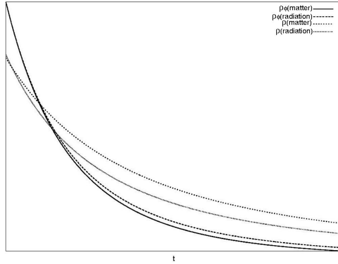
Figure 4: Evolution of energy densities of matter, radiation and the coupled scalar field. The arbitrary constants arising in the integration of Eq.43 have been chosen in order to draw all the curves in the same plot. ( \dot{\phi}_0 = 1 , \ddot{\phi}_0 = -5 , \lambda = 0.1 , k = 0 ).
