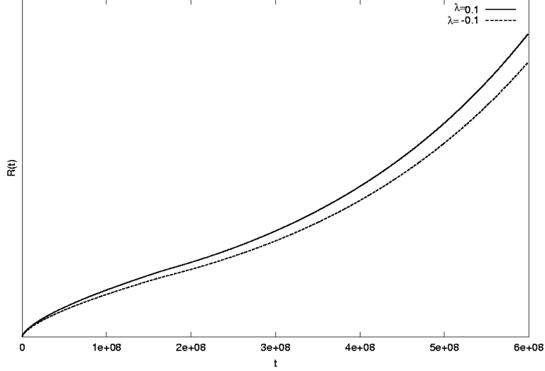
Figure 3: Expansion factor computed from Eqs. 49 and 39 illustrating the behaviour of an hypothetic universe filled with matter ( \omega = 0 ) and an exponentially harmonic map. ( \dot{\phi}_0 = 1 , \ddot{\phi}_0 = -5 , \omega = 0 , k = 0 ).
